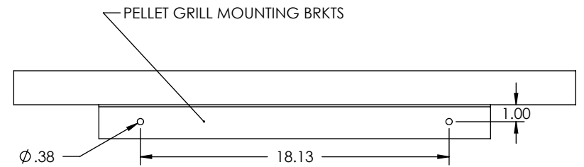
COUNTERTOP SIDE VIEW
